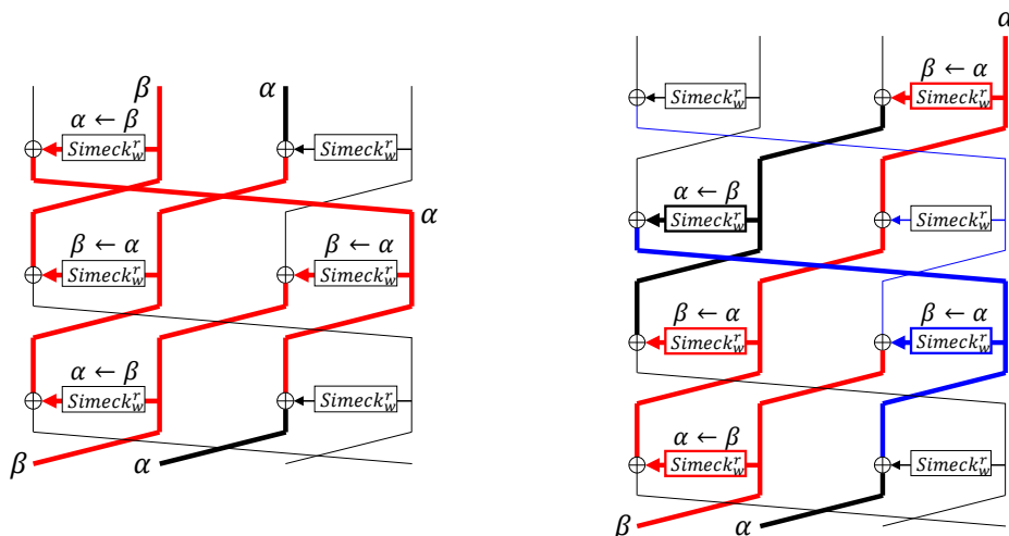
Figure 4: Left: Previous 3-Step Inbound Procedure for sLiSCP. Right: Improved 4-Step Inbound Procedure for sLiSCP. In the previous procedure, four active Simeck boxes are fixed independently, while in the new procedure, fixing three active Simeck boxes (red) will fix another one (blue), and an additional one (black) can be fixed independently.
