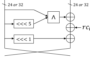
Figure 2: Round Function of Simeck.
