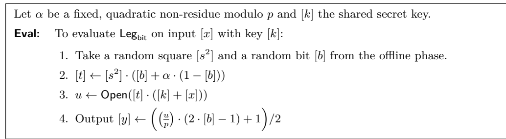
Figure 6: Securely computing the \mathbf{Leg}_{\text{bit}} PRF with secret-shared input and output (Redacted copy of [GRR + 16, Figure 7]).
