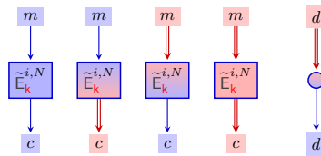
Figure 4: Pictorial notation to define processing of open versus shared data.
