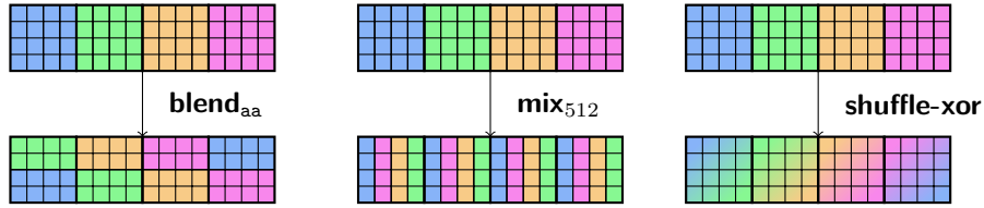
Figure 8: Effect of applying one round of the mixing layers on the state of \pi_{512} .
