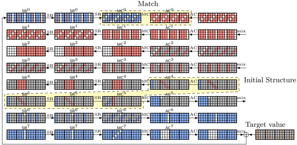
Figure 6: Meet-in-the-middle attack on 4 rounds of Haraka-512 v2. All \square are unknown, \square are constant, \blacksquare neutral bytes backward, \blacksquare neutral bytes forward and \blacksquare are the bytes truncated at the output.
