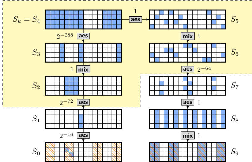
Figure 3: Truncated model utilizing degrees of freedom for T = 3, m = 2 and q = 2 . An active byte is marked as \blacksquare ; a byte which is removed due to trunc is marked with \blacksquare ; boxes \boxed{f} denotes a function f mapping one state to the next, and the number next to it gives the transition probability. For finding a collision, the attacker would have full control over the middle rounds, marked in the highlighted area. As there are only 53 conditions on bytes which all can be fulfilled with the available degrees of freedom the attack costs for an idealized attacker would be 2^{16} .
