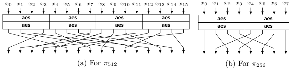
Figure 2: Depictions of round functions R_t for \pi_{512} (a) and for \pi_{256} (b). Each x_i denotes a column of 4 bytes of the state.
