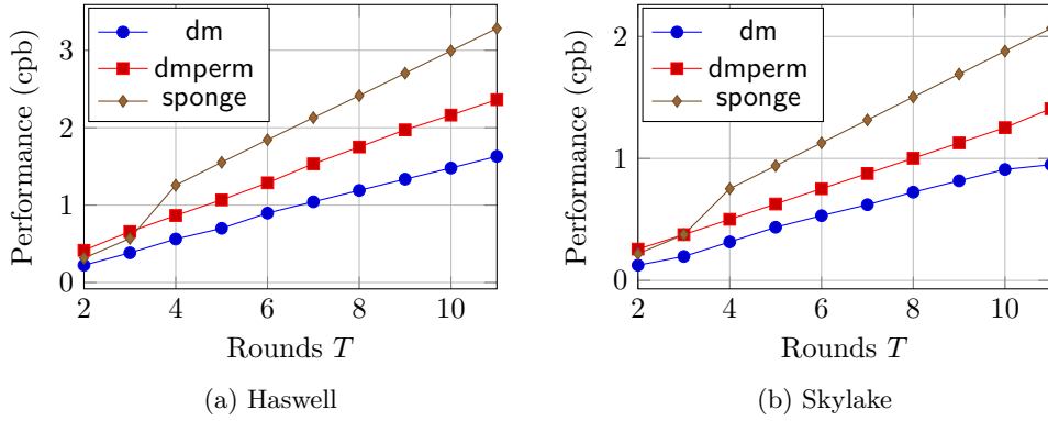
Figure 7: Performance using m = 2 for each of the three general Haraka-512 v2 constructions considered
