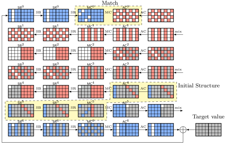
Figure 4: Meet-in-the-middle attack on 3.5 rounds of Haraka-256 v2. All \square are unknown, \blacksquare are constant, \color{red}\square neutral bytes backward and \color{blue}\square neutral bytes forward.
