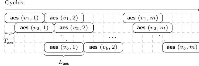
Figure 5: Pipelined AES instructions. A box \text{aes}(v, i) denotes the application of the i th AES round to a block v .
