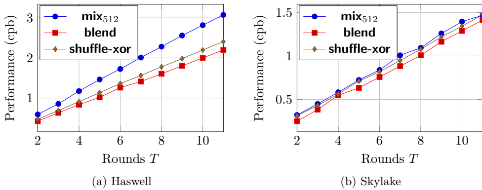
Figure 9: Performance of Haraka-512 v2 using m = 2 for each of the three approaches to linear mixing considered
