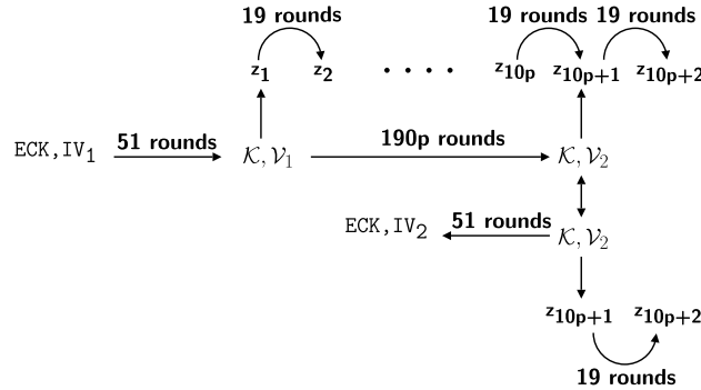
Figure 3: Generating \text{IV} pairs that produce shifted keystream bytes.
