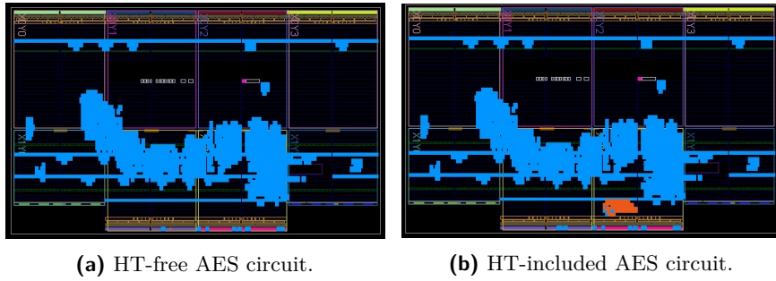
Figure 15: Genuine (HT-free) and HT T1100-included AES circuits.
