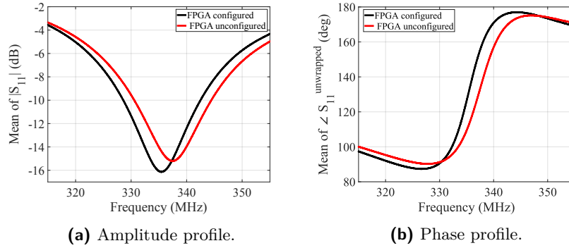
Figure 9: The mean of reflection response of the chip for the configuration mode of the FPGA over 315 MHz - 355 MHz.
